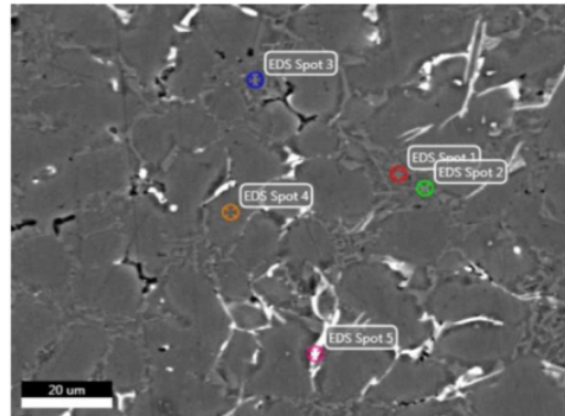
Figure-8. EDS micrograph aluminum alloys ADC12 (Stirred slurry aluminum) at pouring temperature 600 °C.
