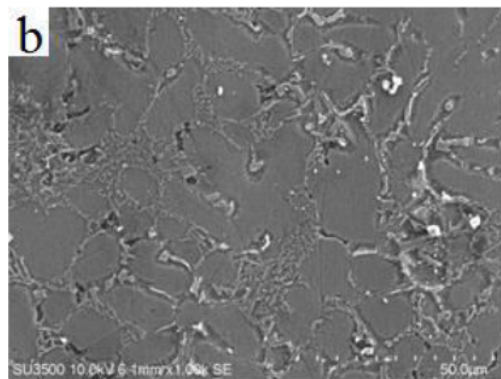
Figure-7. SEM micrograph aluminum alloys ADC12, (a) Unstirred slurry aluminum, (b) Stirred slurry aluminum, (1000X magnification) at pouring temperature 600 °C.
