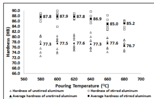
Figure-2. The hardness of ADC12 aluminum alloys at semi-solid casting.
